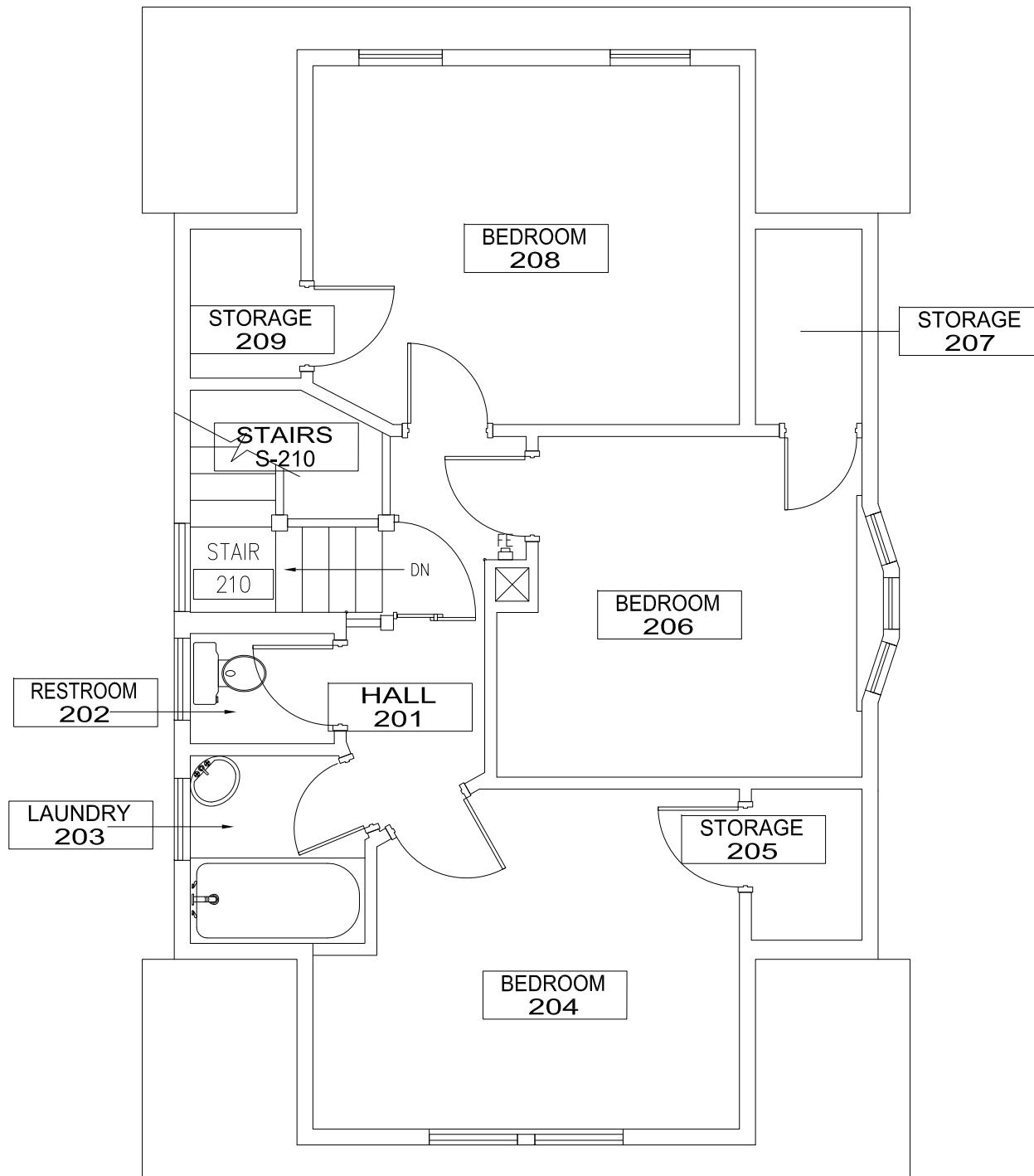
366 - Women's Transition 3 SECOND FLOOR - BASE
