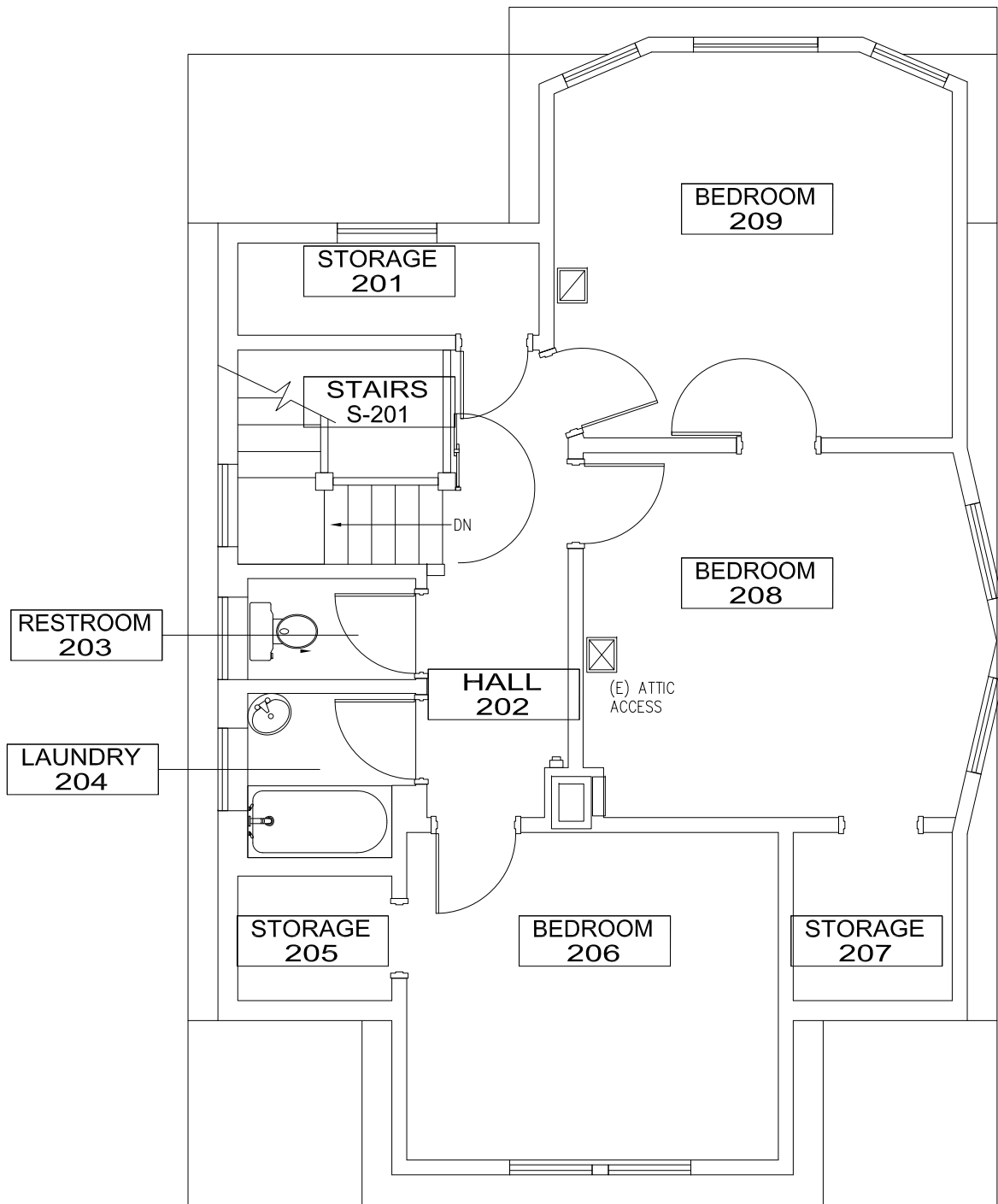
360 - Women Transition 1 SECOND FLOOR - BASE
