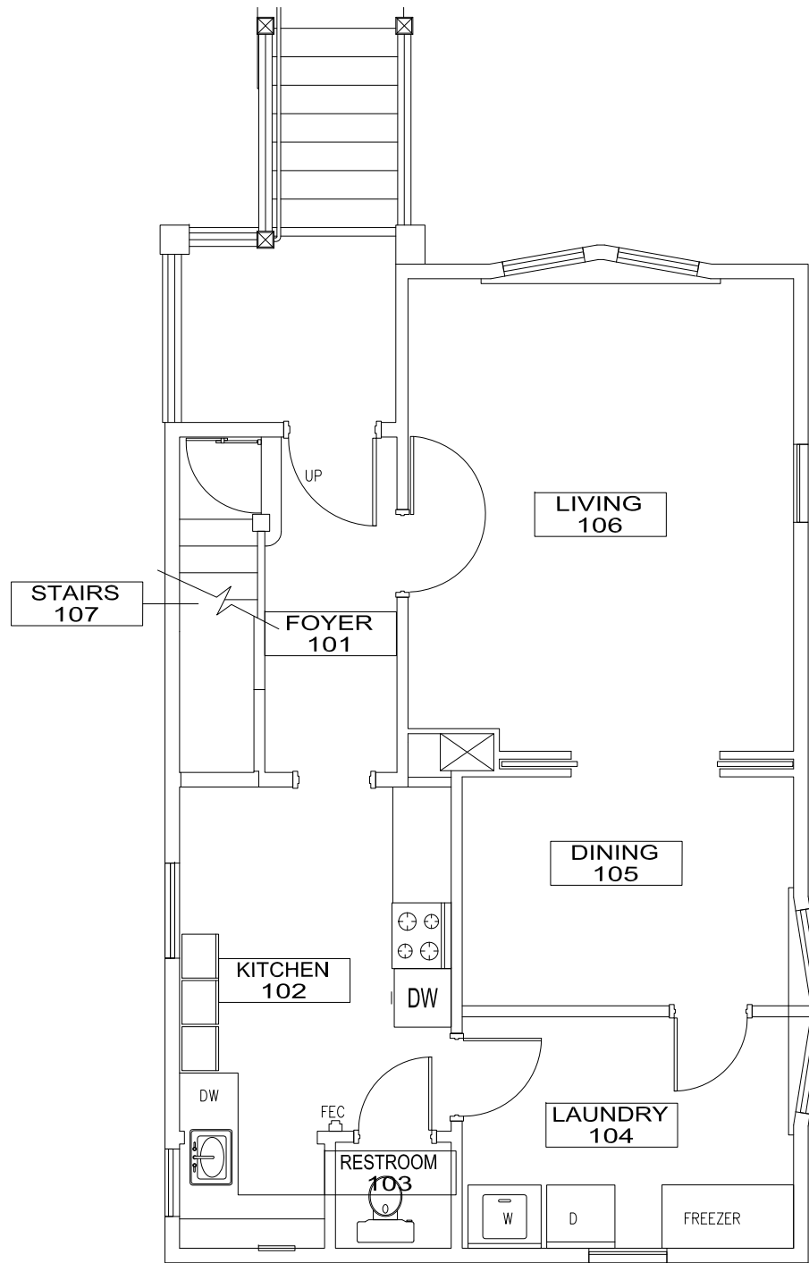
366 - Women's Transition 3 FIRST FLOOR - BASE
