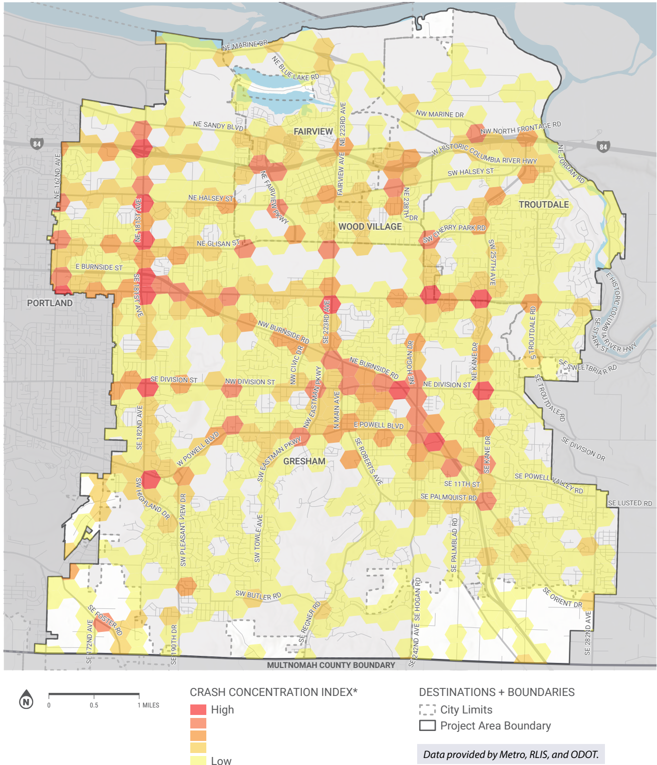
Figure 10. Vehicular Crashes, 2013-2022
