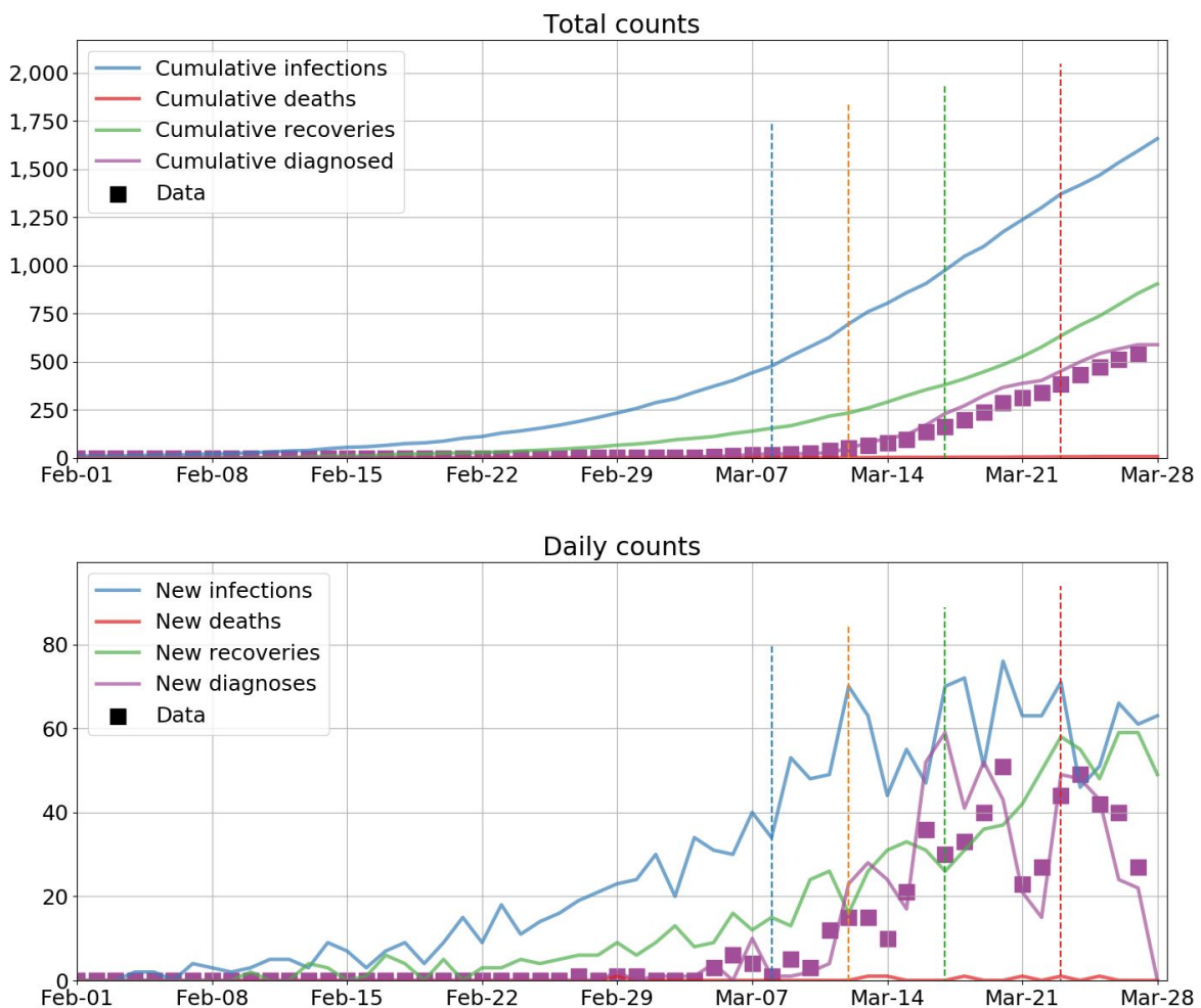
Figure 1: Revised model calibration with the latest case data, showing the timing of different interventions, and approximately 1,750 infections (80% forecast interval: 1,200 to 3,000) by March 28th. Dotted lines correspond to reductions in transmission relative to baseline, from left to right, of 10%, 20%, 35%, and 55%. The impacts of these interventions were estimated by calibrating to numbers of positive diagnoses (dots), deaths, and hospitalizations (not shown).
