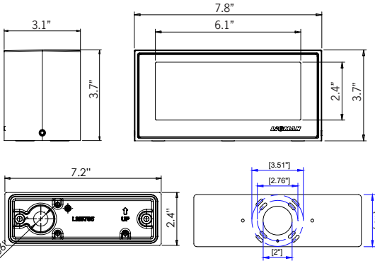
Mounting Detail
