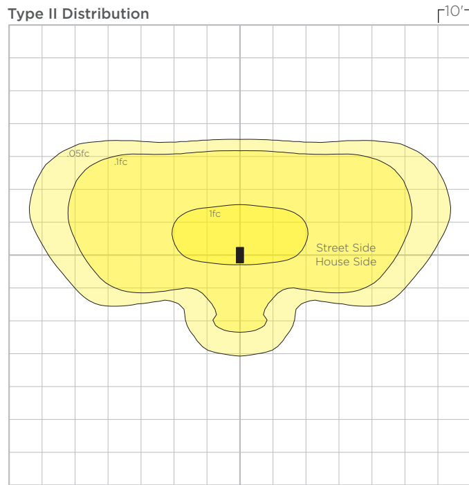
LINW-M1100-L27-2-C(X)-UNV-XX-STD mounted at 16'
