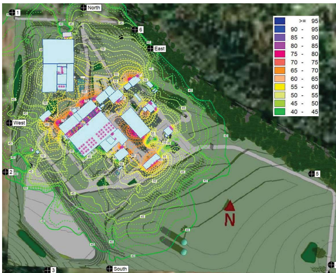
Figure 4. Noise Contours; Bull Run Filtration Facility-No Emergency Generator
