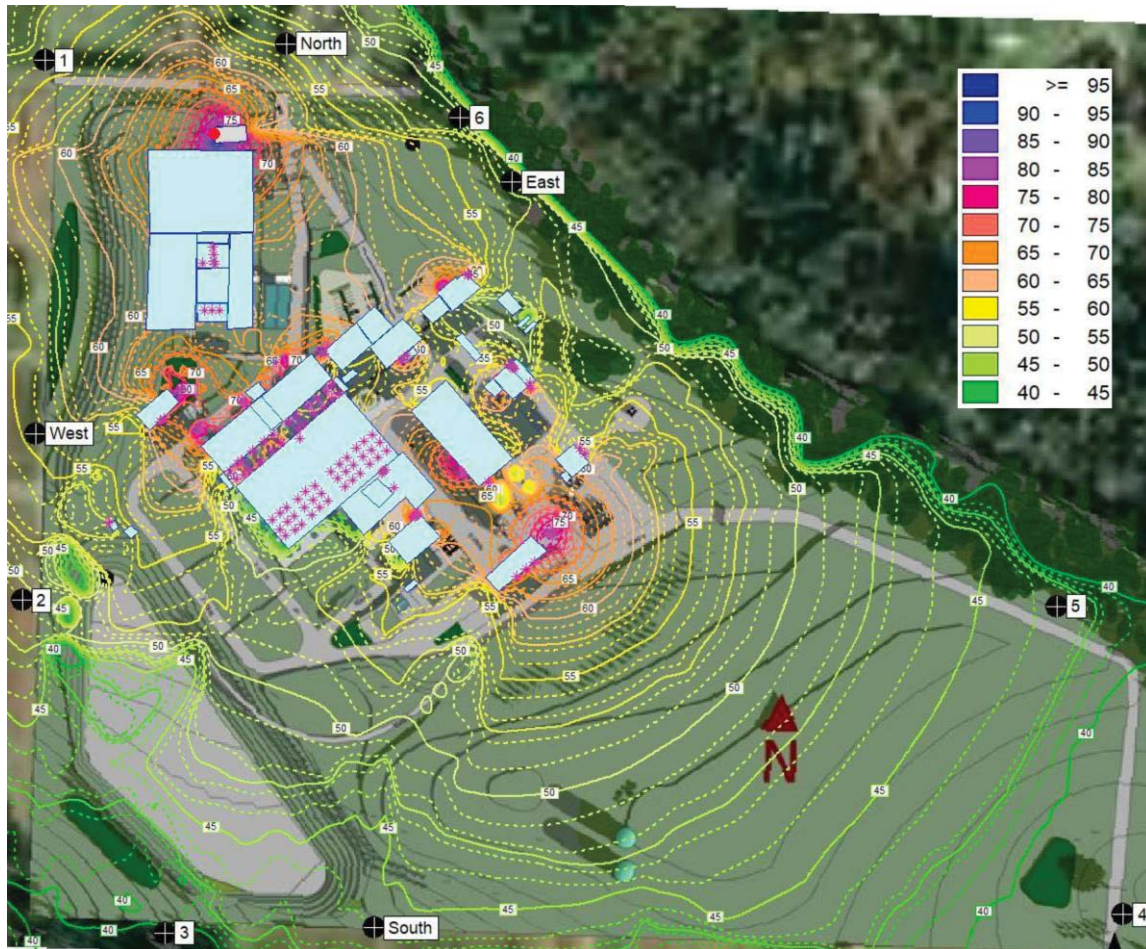
Figure 5. Noise Contour; Bull Run Filtration Facility During Generator and Fire Pump Daytime Testing.
