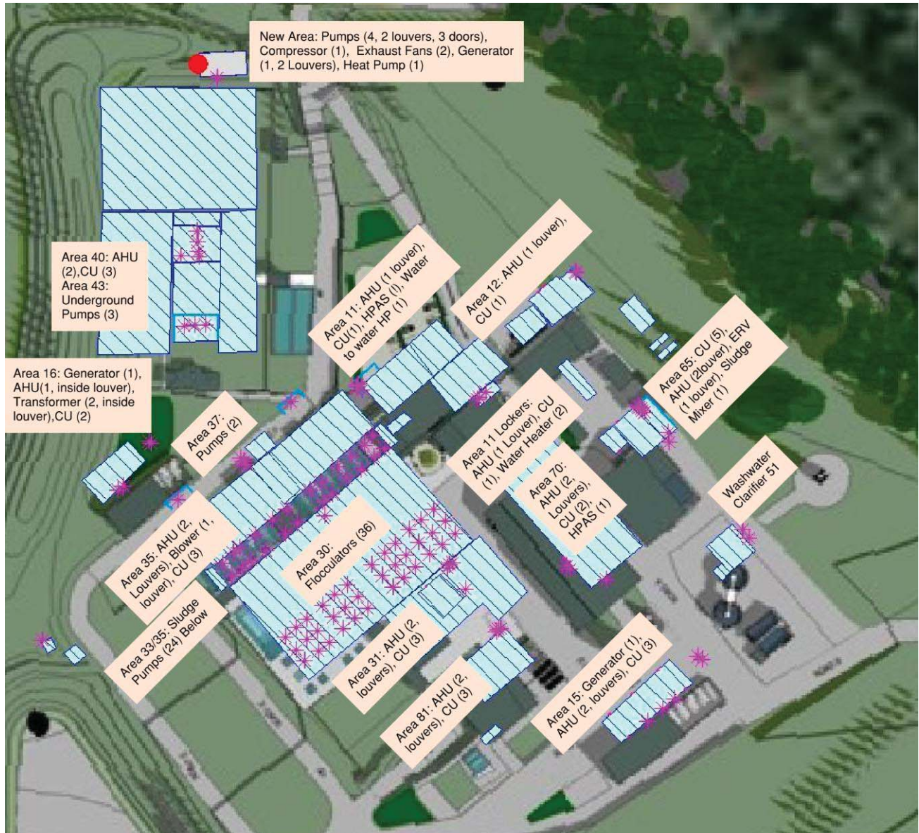
Figure 2. Source Locations (Pink Stars and Red Dots) for Noise Analysis
