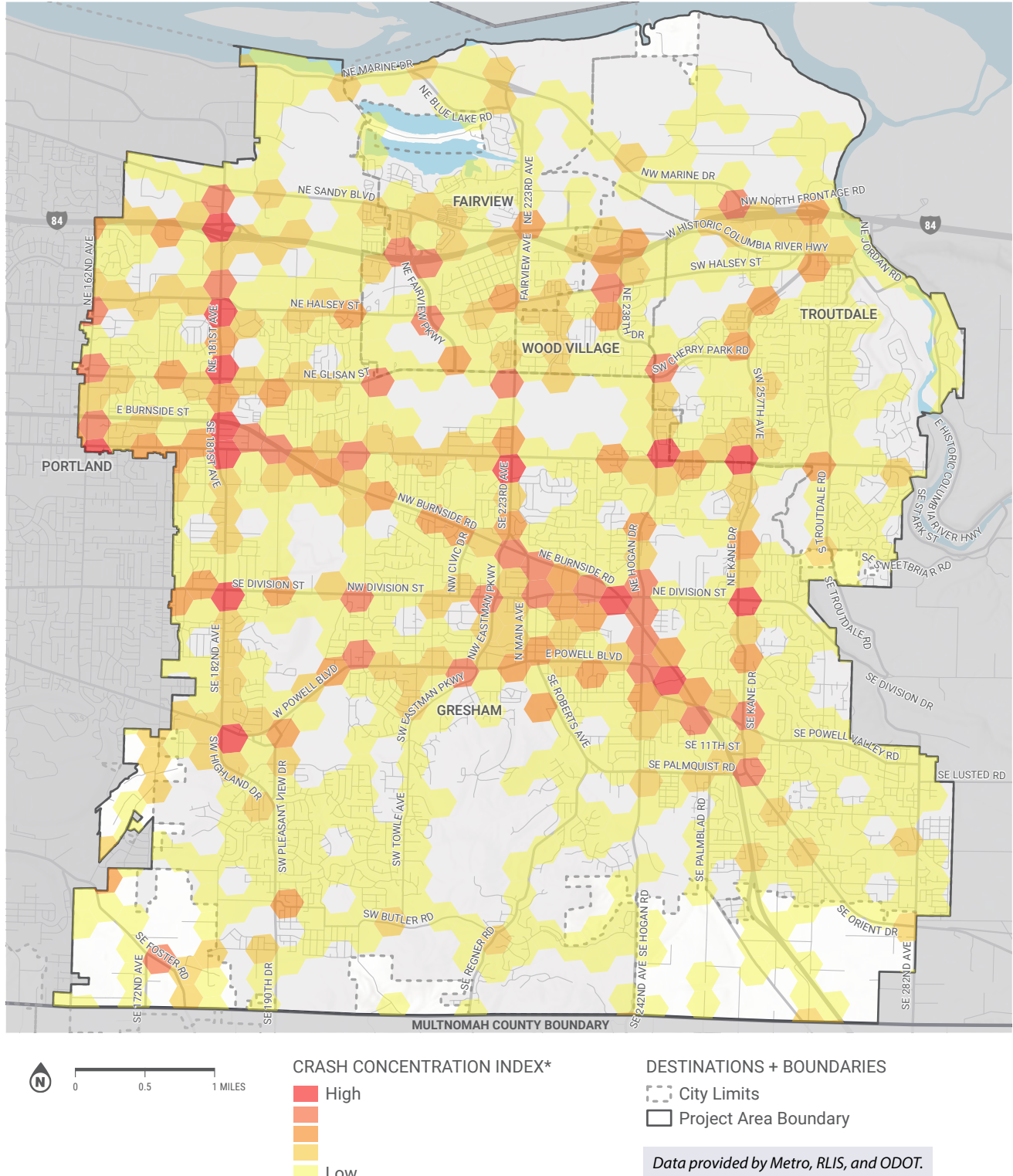
Figure 10. Vehicular Crashes, 2013-2022
