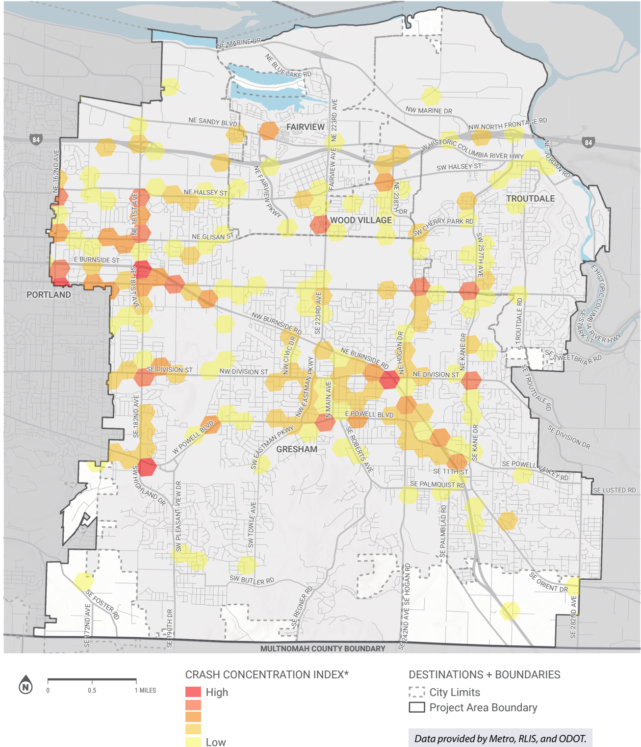
Figure 8. Pedestrian Crashes, 2013-2022
