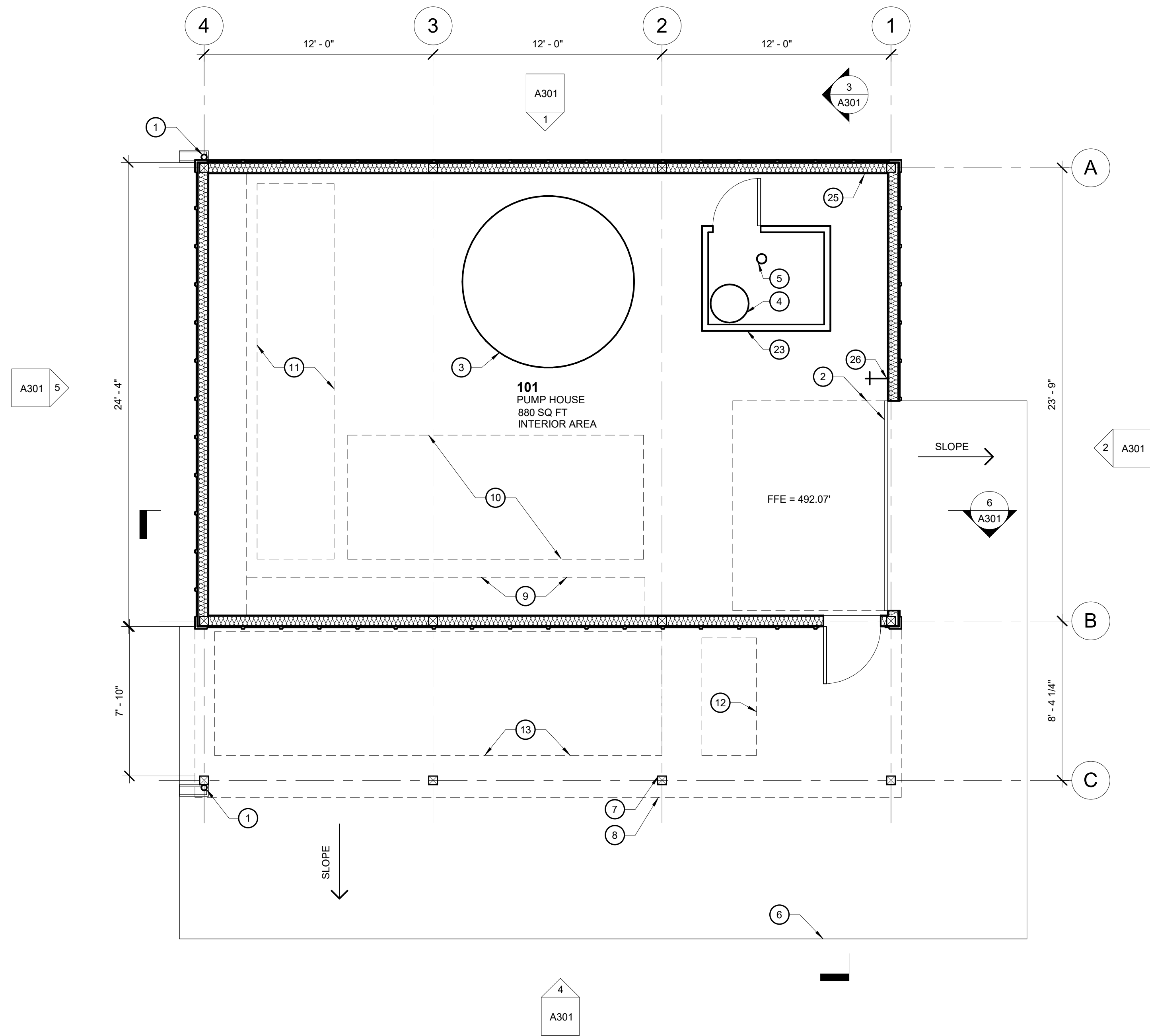
FLOOR PLAN - LEVEL 1 1/4" = 1'-0" 1
