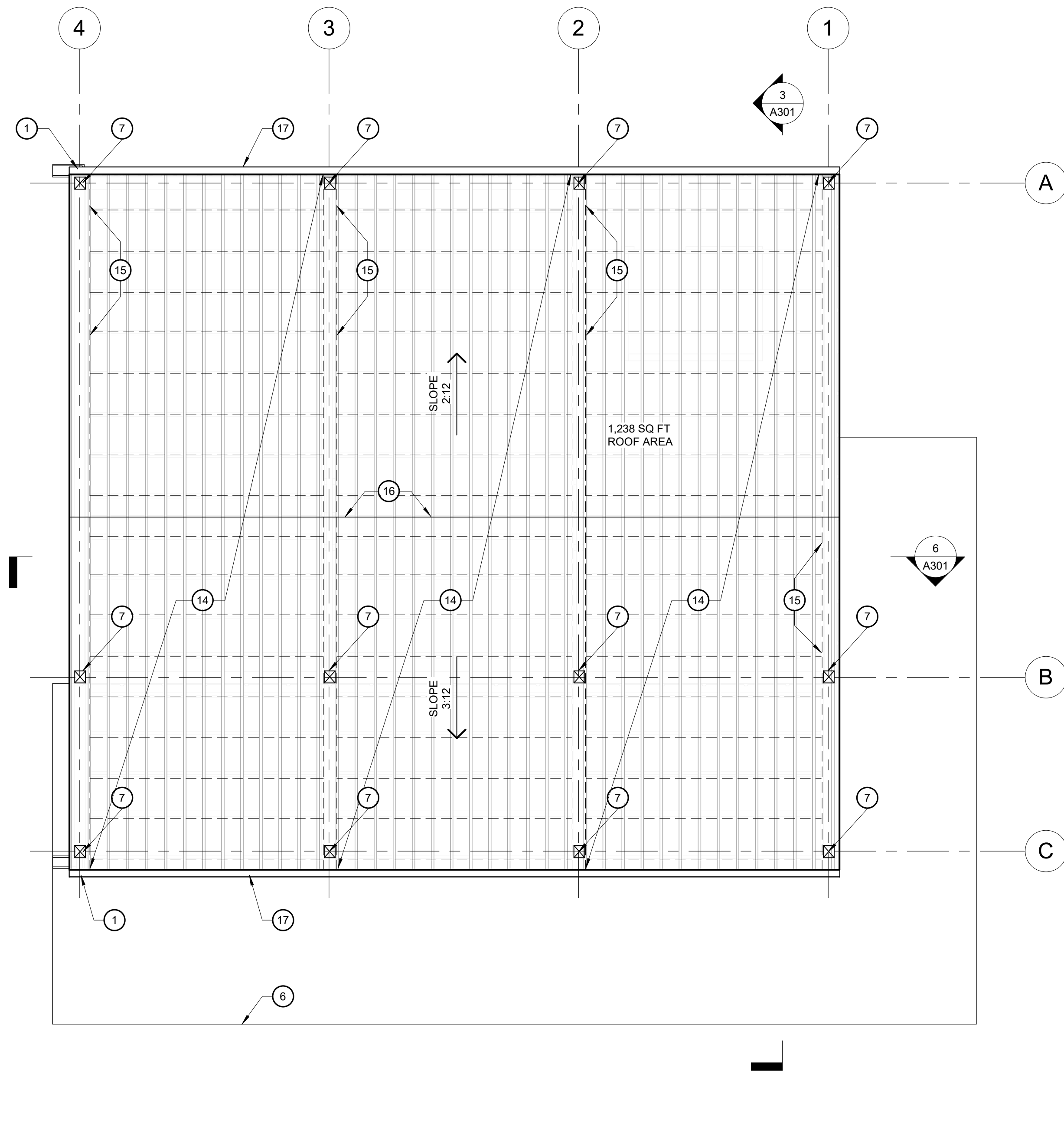
ROOF/BUILDING FRAMING PLAN 1/4" = 1'-0" 2
