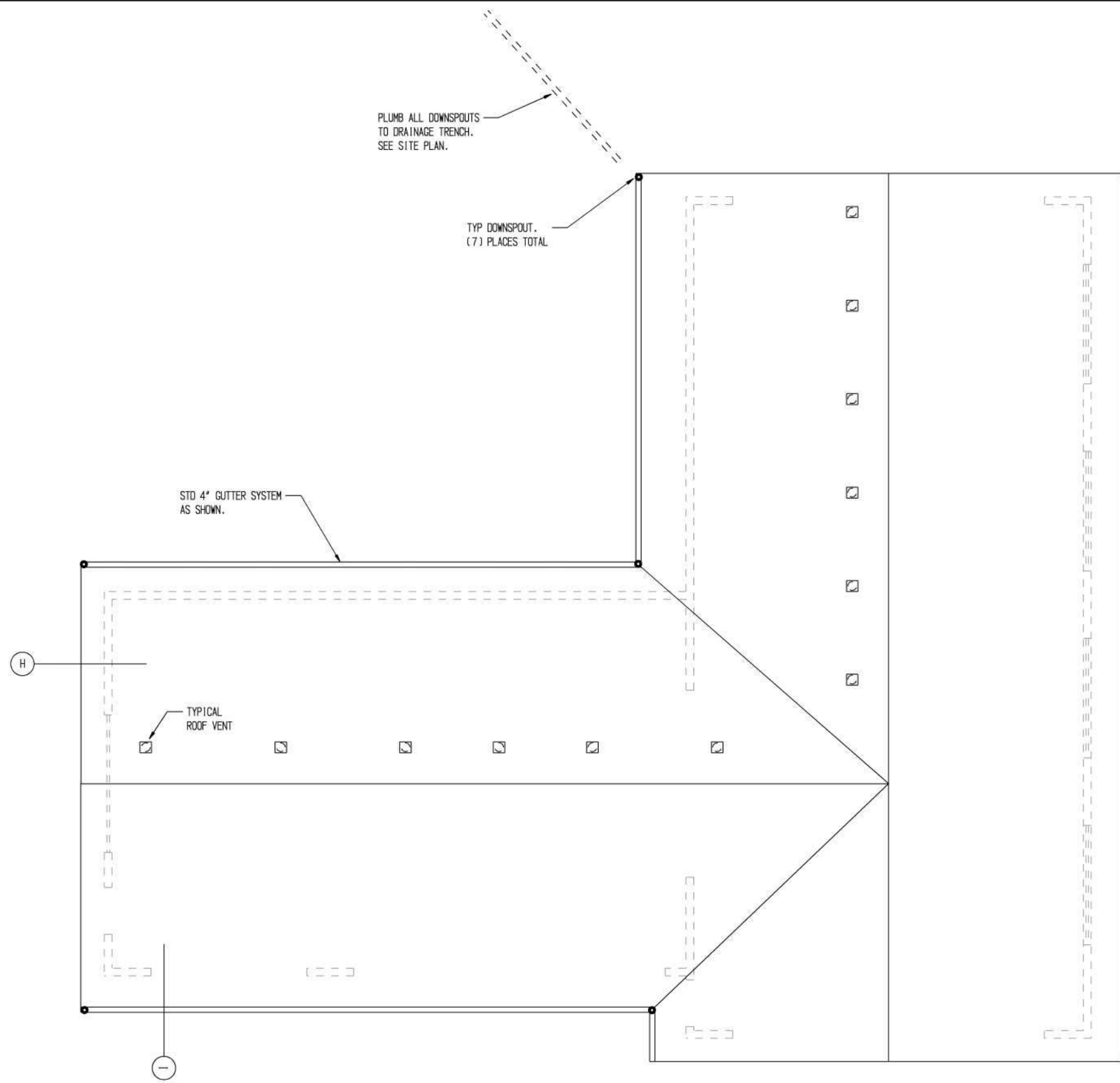
E ROOF/FLOOR PLAN 1/8" = 1'-0"
