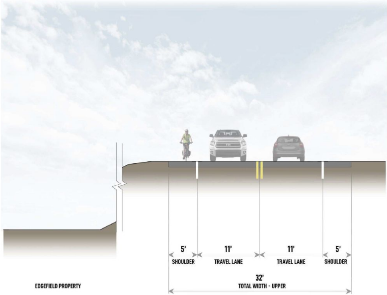
EDGEFIELD - EXISTING SECTION
